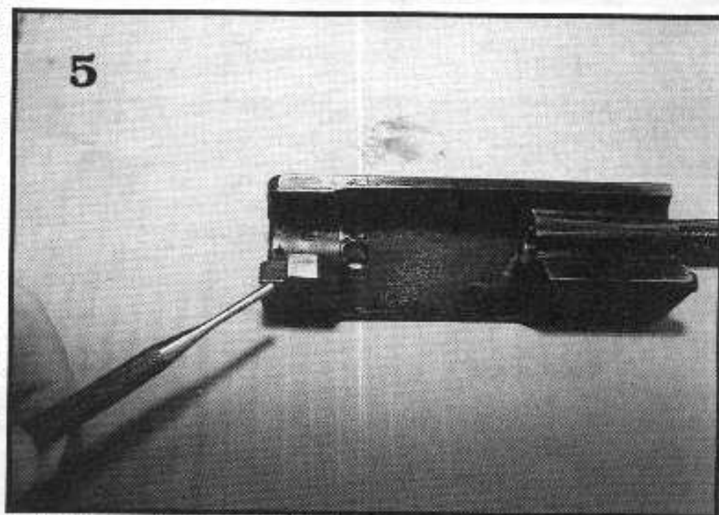
Sear engagement surface on M10 bolt.
