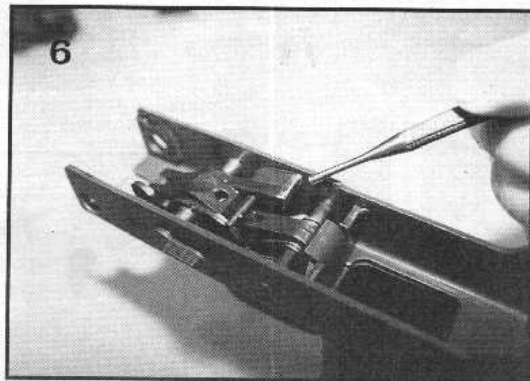
Above: Check this edge of sear for burrs.
